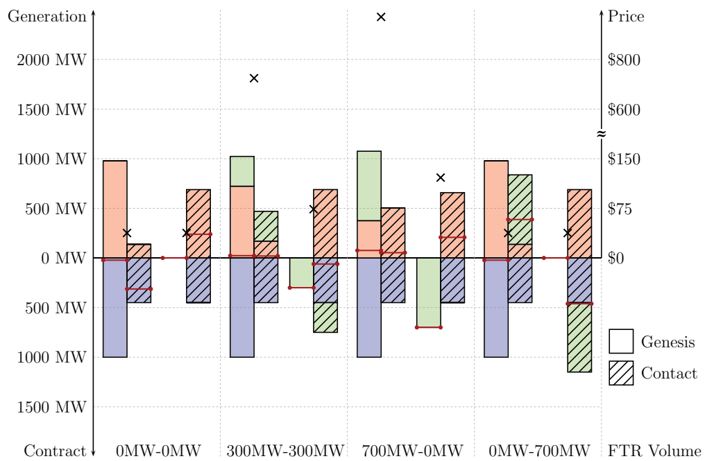
Figure 9: Cournot game with FTRs from BEN-HAY; period 19 of 3 Nov 2008.
